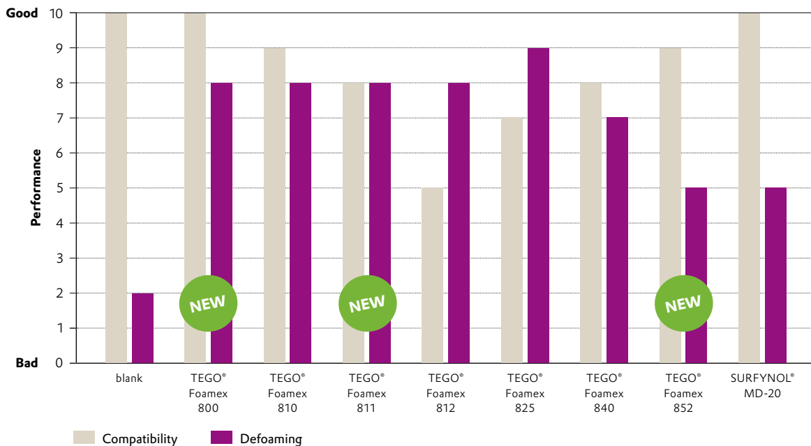
Defoamer positioning in a leather coating
