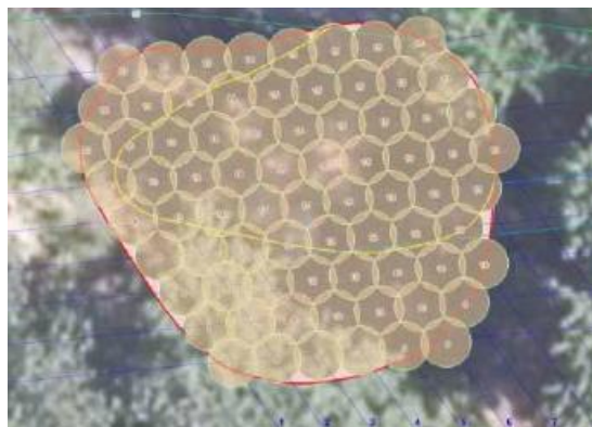
Figure 1 | Layout of soil mixing columns with overlap
