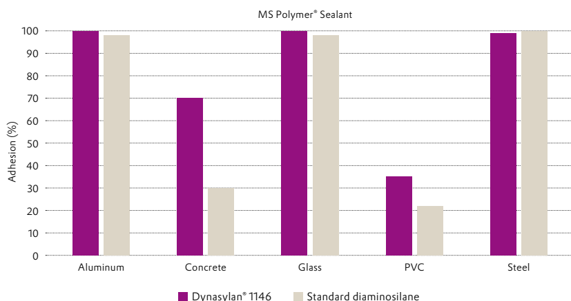
Adhesion performance of MS Polymer® Sealants on various substrates
