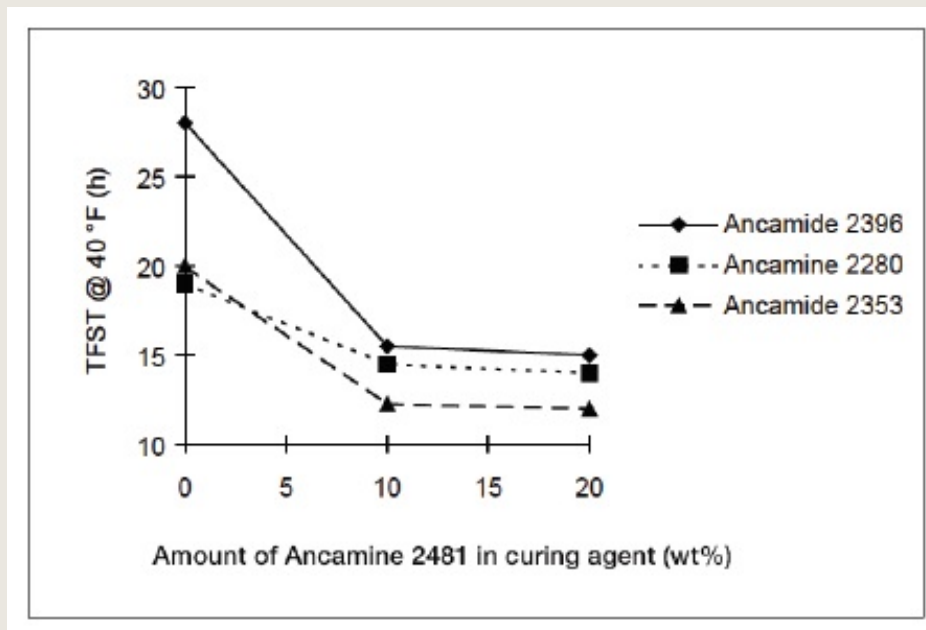
FIGURE 2: ACCELERATION WITH ANCAMINE 2481 CURING AGENT AT 40°F
